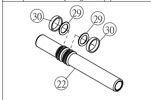
22-30|ShaftOfDiaphragm Set|1|DS03-22-30
