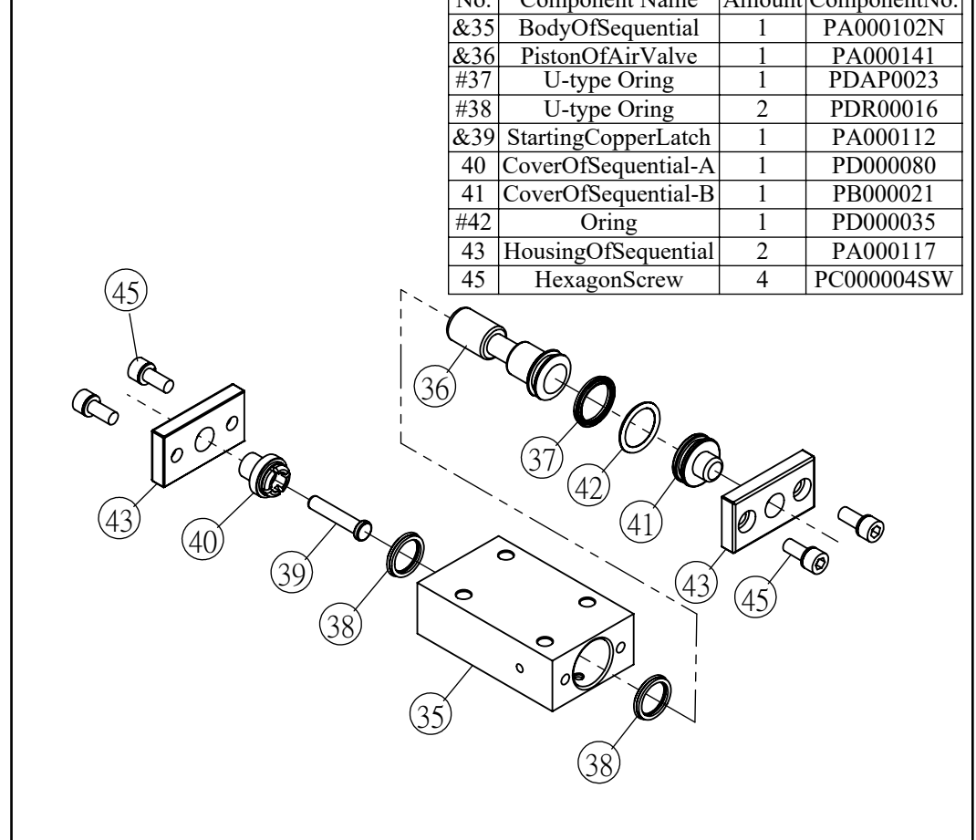
35-45|Air-Valve Set|1|DS03-35-45
